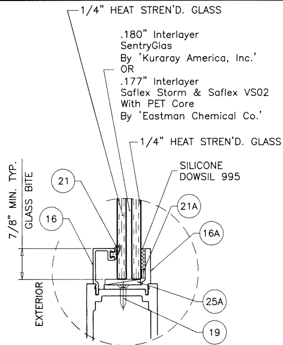
GLASS TYPE 'E2' 11/16" OVERALL LAM. GLASS
