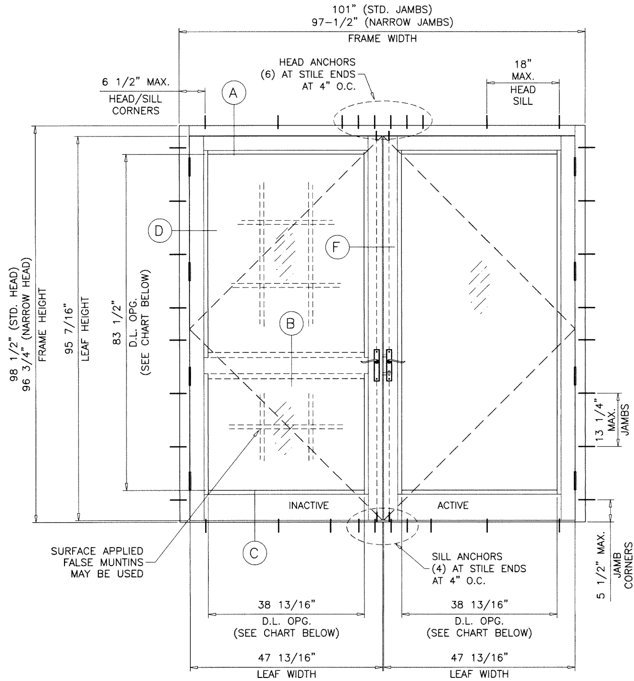
TYPICAL ELEVATIONS
