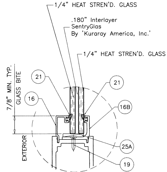
GLASS TYPE 'E3' 11/16" OVERALL LAM. GLASS
