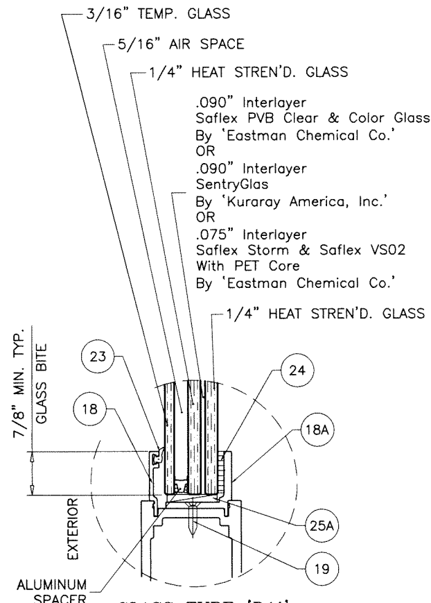
GLASS TYPE 'D1i' 1-1/16" OVERALL INSUL. LAM. GLASS
