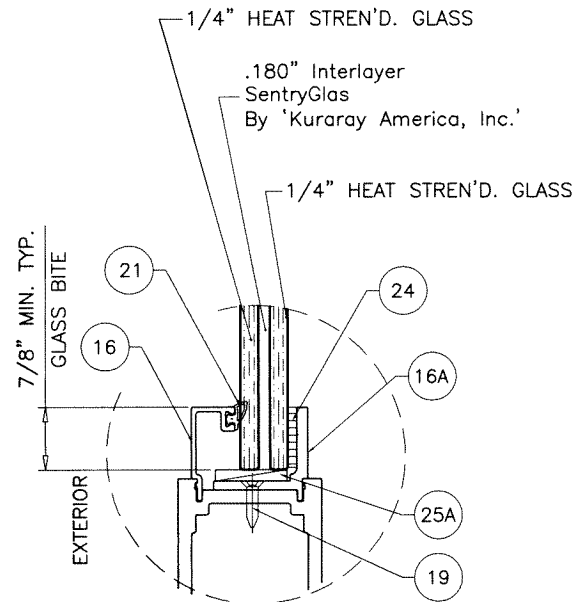
GLASS TYPE 'E1' 11/16" OVERALL LAM. GLASS
